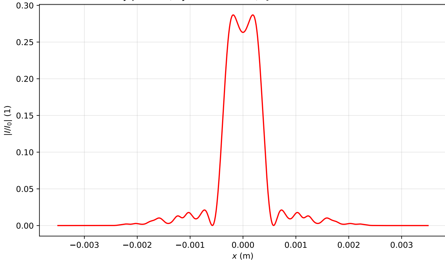
Intensity profile I(x, y = 0, z = 3.981)/I_0 , P_{in}=4.0P_{cr} , artificial time
